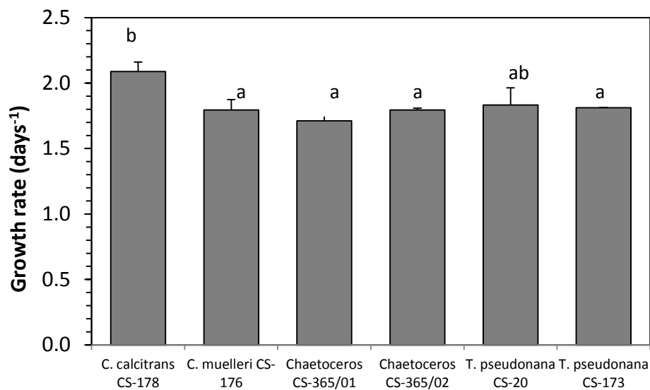
Figure 7.4.3: Mean ( \pm SE) growth rate of candidate algal strains grown in 20L carboys ( n=2 , 20-22°C, 150 \mu\text{moles photons PARm}^{-2} \text{s}^{-1} at carboy surface). Means with different letters are significantly different from one another.
