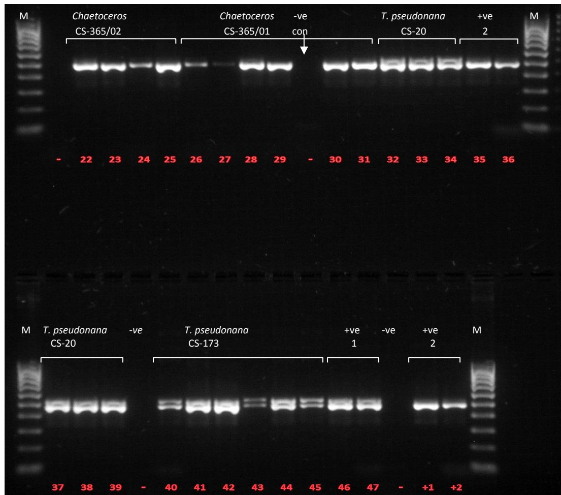
Figure 7.4.1: Detection of bacterial ribosomal RNA genes from 22 plate-purified subclones of the four candidate species. (–ve)=negative control; (+ve1)=DNA extracted from original bacteria contaminated cultures; (+ve2)=DNA extracted from a known non-axenic algal culture of a different species).
