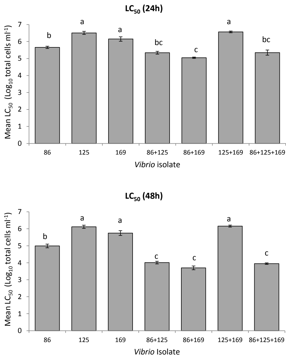
Figure 7.3.11: Virulence (LC 50 ± SE, Log cells mL -1 ) of three hatchery Vibrio isolates to 17-20 day old mussel pediveligers in 24 and 48h pediveliger challenge assays. Isolates were assayed singly and in combination at equal concentration. Letters indicate significantly different means.
