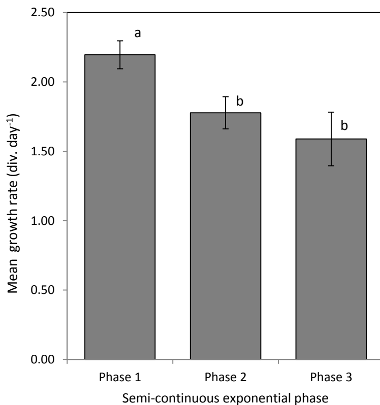
Figure 7.4.5: Mean exponential growth rate ( \pm SE) of candidate strains over three semi-continuous growth phases in 40L polyethylene hanging bags (20-22°C, 120 \mu moles photons m^{-2} s^{-1} at bag surface). Means with different letters are significantly different from one another.
