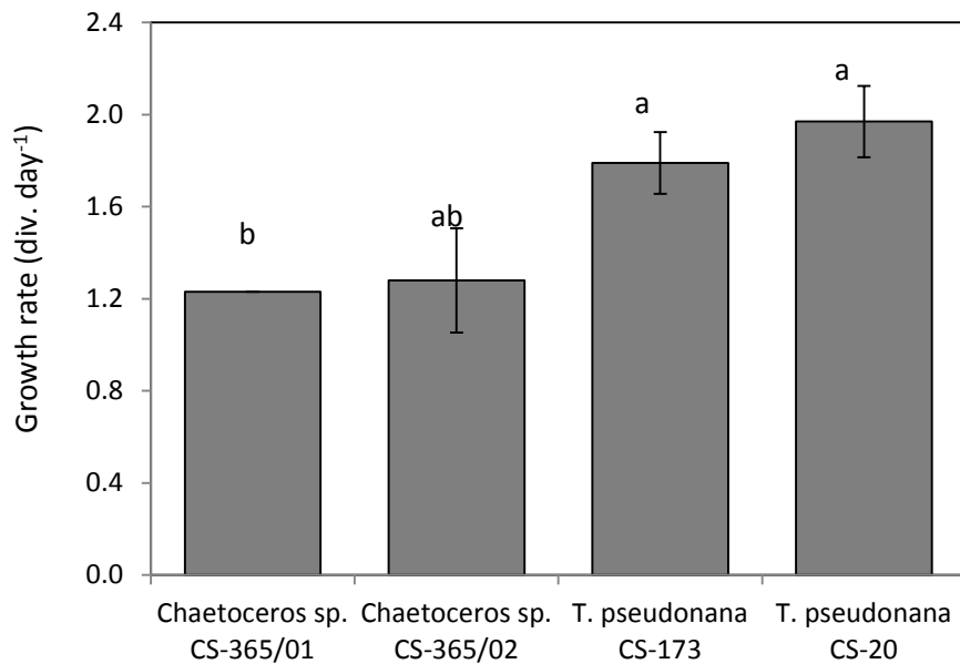
Figure 7.4.9: Mean growth rate of candidate species over three growth phases in 40L hanging bags. Bags were grown under semi-continuous culture conditions (20-22°C, 120 \mu\text{moles photons m}^{-2} \text{s}^{-1} at bag surface). Means with different letters are significantly different from one another.
