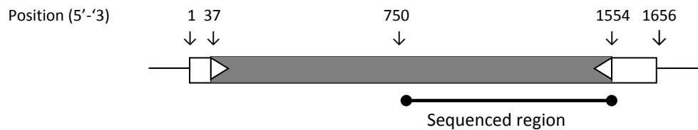
Figure 6.3.2: The region of atpA gene amplified using PCR primers atpA37F and atpA1554R (grey shading) producing a PCR amplicon size of approx. 1500 bp. White triangles indicate the relative position of the amplification primers. The 800bp region sequenced using the reverse amplification primer is indicated.
