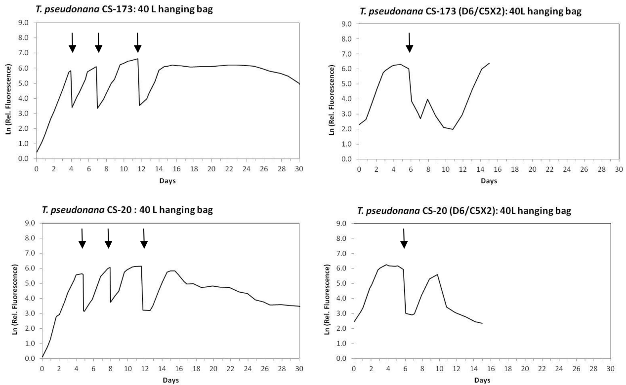
Figure 7.4.7: Growth dynamics of Thalassiosira pseudonana strains in 40 L hanging bags under semi-continuous culture conditions (20-22°C, 120 \mu\text{moles photons m}^{-2} \text{s}^{-1} at bag surface) prior to (left) and after (right) antibiotic purification to reduce/remove bacterial community. Arrows indicate to 90% harvest and media replacement. Note that post-purification growth experiments were terminated at 15 days after two growth/harvest cycles.
